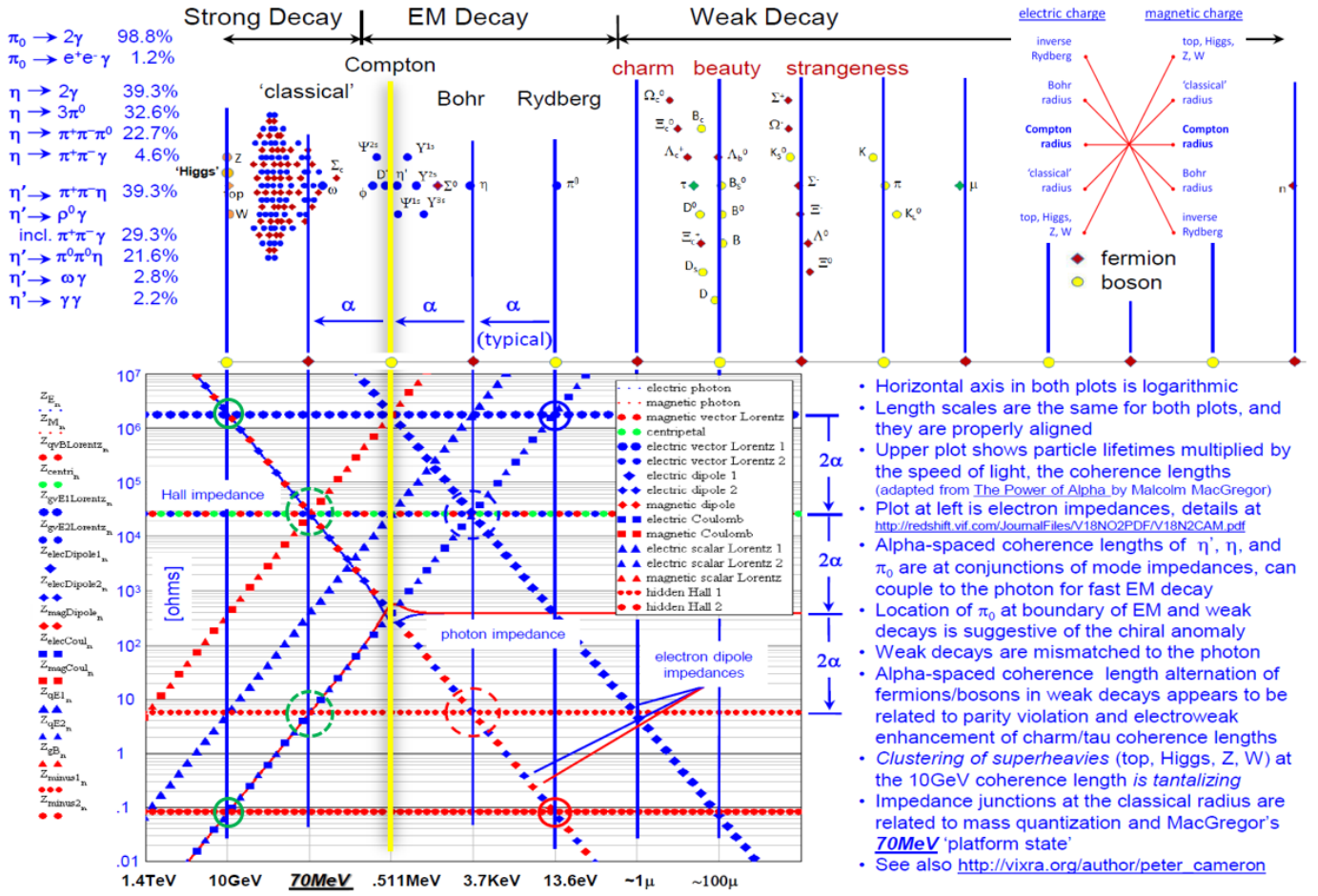
FIG. 1: BSM origin of unstable particle lifetimes in terms of quantized impedance networks of GWI. Dynamic SUSY of alternating fermion and boson lines in weak decays has its origin in topological symmetry breaking of the neutrino, as indicated by topological inversion of magnetic charge at upper right[37].
